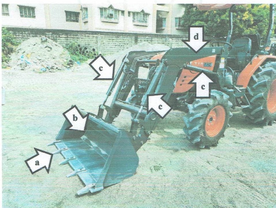
Figure 1. Parts of the HANIL HL25 Front Loader mounted to 40.5 kW TYM 5825R Four-Wheel Tractor include the following: (a) Ground-engaging tool, (b) Bucket, (c) Hydraulic cylinders, and (d) Arm.
